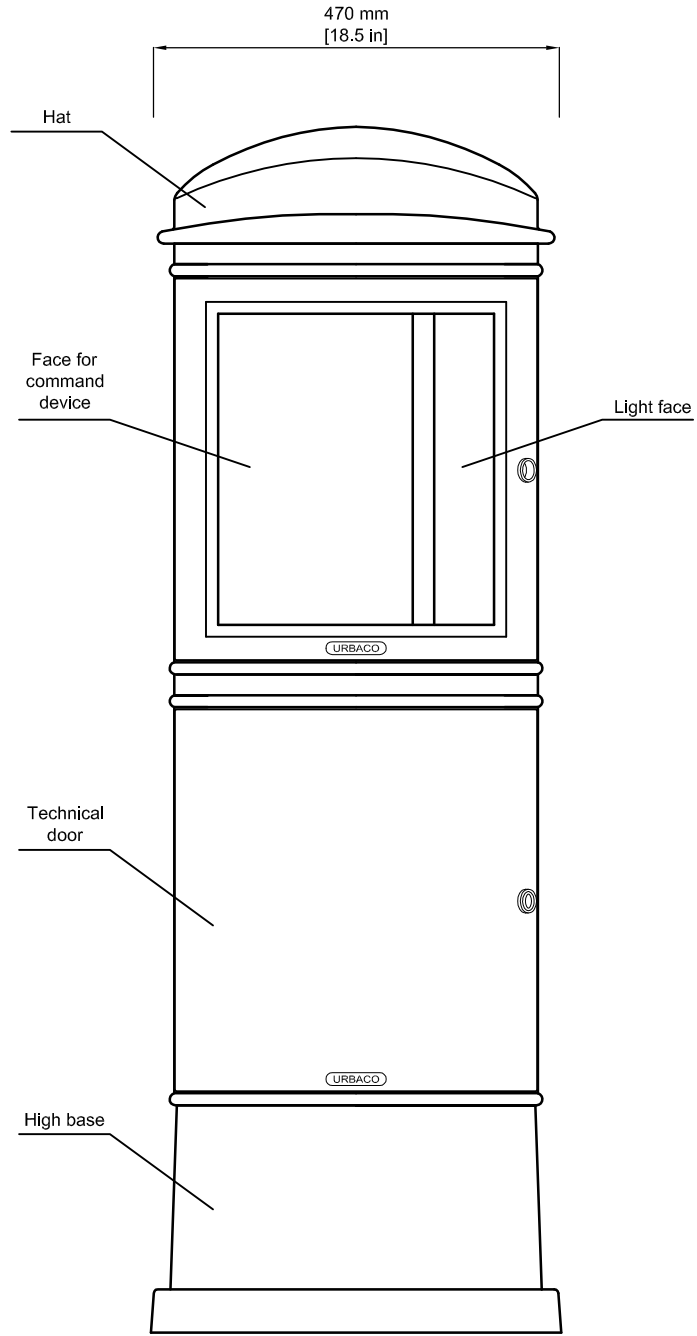
Front view
