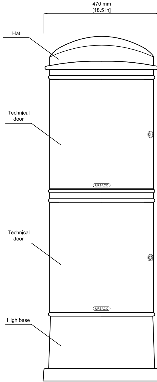
Front view
